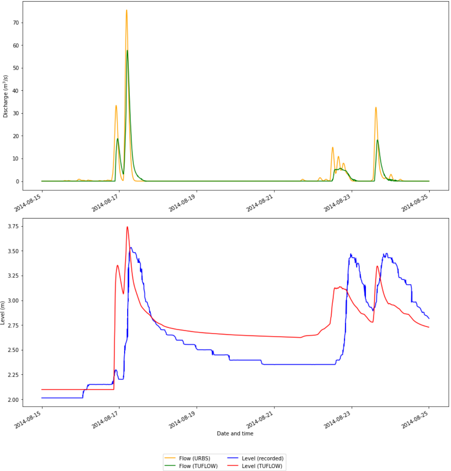
Figure 8-1 2014 Booral Road Alert Calibration Plots
